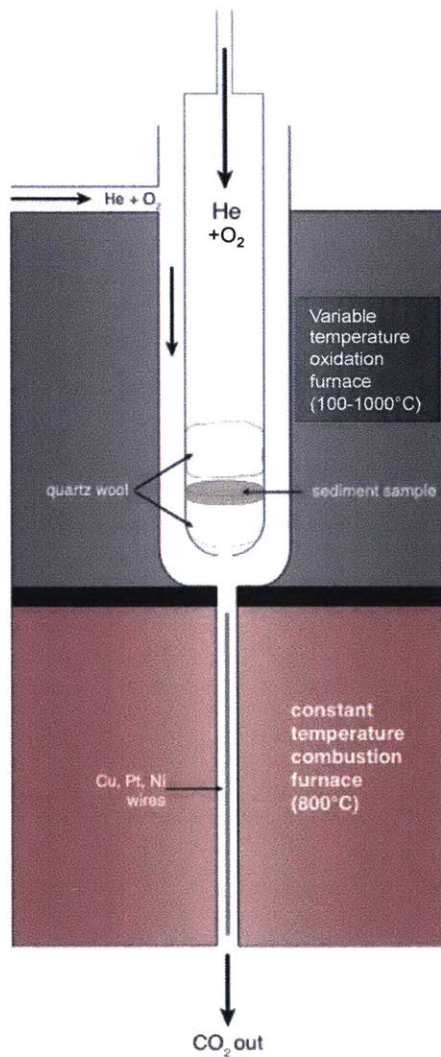
Figure 1. Schematic of the ramped pyrolysis/oxidation (RPO) unit at the National Ocean Sciences Accelerator Mass Spectrometry facility at WHOI. Adapted from (Fornace, 2016).
