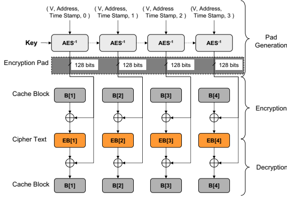
Figure 4: Encryption mechanism that uses one-time-pads from the AES algorithm with time stamps.
